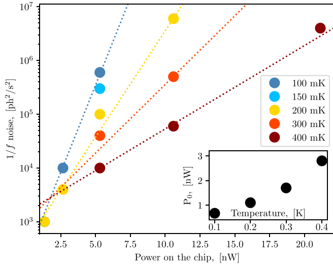
FIG. 6. A_f constant of 1/f noise contribution fitted at different powers and temperatures, in units of photons on chip. Dashed lines are exponential fits: A_f = A_0(T)e^{P/P_0(T)} (see text). Inset: P_0 fit parameter from the main graph as a function of temperature T .
