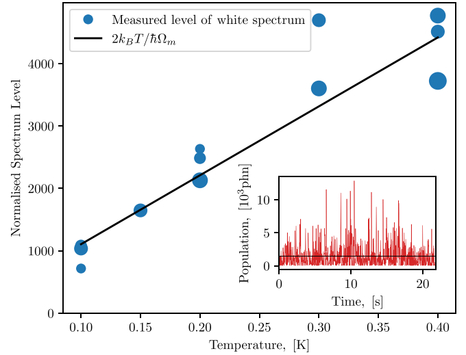
FIG. 5. Normalized spectrum level (no units) \sqrt{\frac{\Gamma_m S_0}{\mathcal{G}^2}} / (\frac{\kappa_{\text{ext}}/2}{\kappa_{\text{tot}}} |\Gamma_{\text{opt}}|) at different temperatures and pump powers (size of dots from small/low to big/large P_{\text{in}} ). The line is the theoretical calculation with no free parameters (see text). Inset : Time trace of population fluctuations at the fastest acquisition speed (200 mK, power 10 nW); the line is the mean value; resolution is about 100 phonons; see text for discussion.
