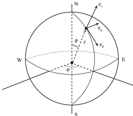
Figure 1. Spherical coordinates.
