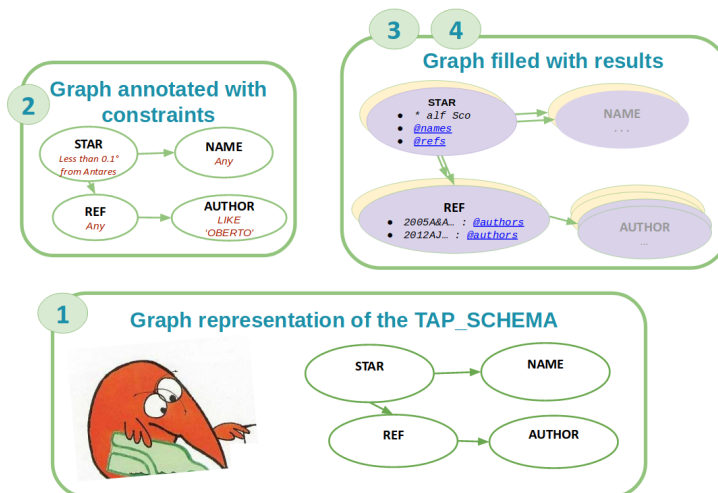
Figure 1. Example on how to query SIMBAD with a TAP graph representation.
