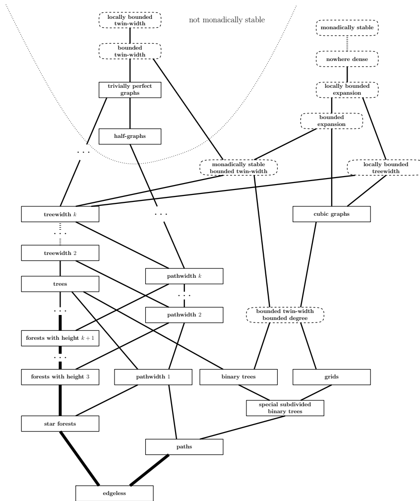
■ Figure 1 Partial outline of the FO transduction quasiorder. The special subdivided binary trees are those subdivisions of binary trees that are subgraphs of the grid. Dashed boxes correspond to families of not necessarily transduction equivalent graph classes sharing a common property. Fat lines correspond to covers, normal lines correspond to strict containment \sqsubset , dotted lines correspond to containment (with a possible collapse). Some parts of Figure 1 will be refined in Figure 2.
