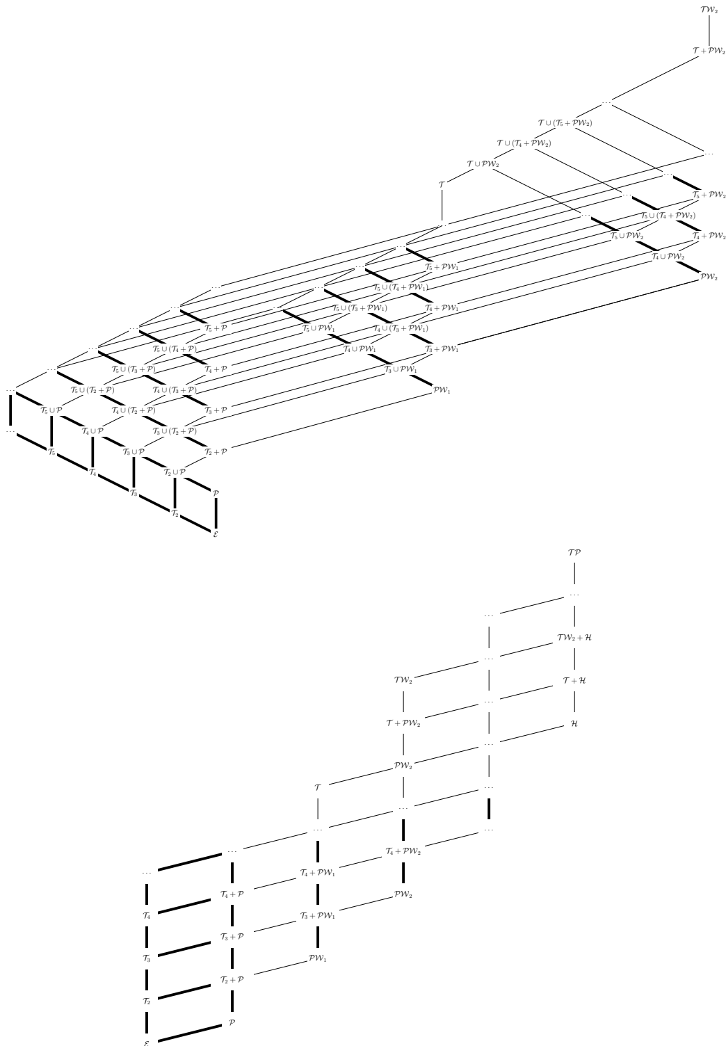
■ Figure 2 A fragment of (\mathcal{C}, \subseteq_{FO}) (top) and a fragment of (\mathcal{A}, \subseteq_{FO}) (bottom). Thick edges are covers.
