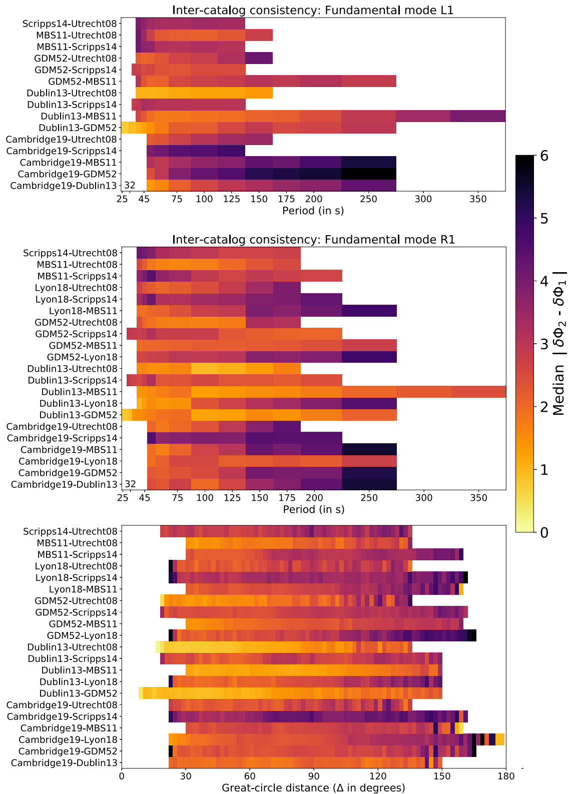
Figure 7. Inter-catalogue consistency between pairs of fundamental-mode dispersion catalogues. Median absolute deviations in reported measurements ( |\delta\phi_2 - \delta\phi_1| ) are plotted at various reference periods for (a) Love and (b) Rayleigh waves. Median values for 100 s Rayleigh waves binned every 2^\circ epicentral distance are provided in (c), while the values for Love waves are provided in Fig. 8.
