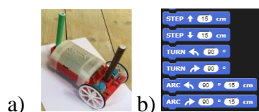
Figure 1: a) view of the GGBot; b) SNAP! Commands list
