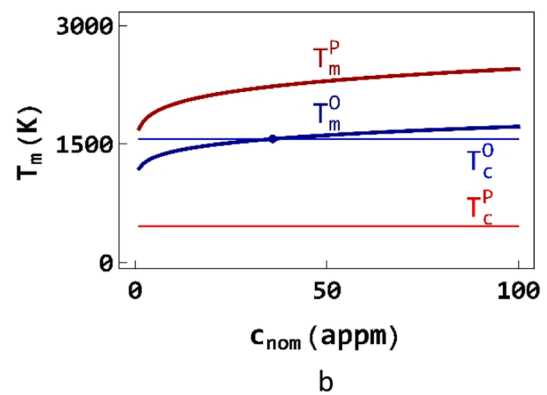
Fig. 5. Evolution of c_P (in red), c_1 (in blue) and c_2 (in green) concentrations with respect to the temperature for c_{nom} = 10 (light circles) and 100 (dark crosses) apm (a), Evolution of the temperature corresponding to c_X = 0.5 , with X = P : T_m^P (dark red) and X = O : T_m^O (dark blue) as a function of the nominal concentration, critical temperatures of the P line (in red) and O line (in blue) are recalled (b). (For interpretation of the references to colour in this figure legend, the reader is referred to the web version of this article.)
