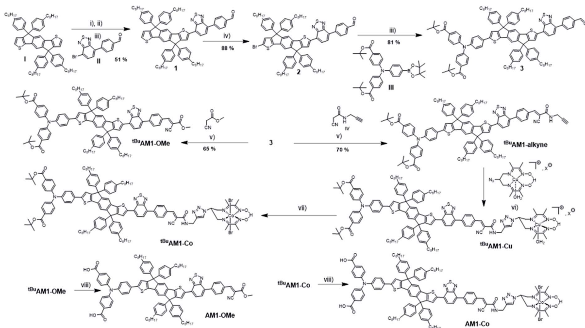
Fig. 2 Synthetic routes and intermediates towards AM1-alkyne and AM1-OMe dyes and AM1-Co dyad, conditions: (i) n -BuLi, THF, -78^{\circ}\text{C} , 1 h; (ii) ^i\text{PrO-Bpin} , THF, RT, 2 h; (iii) \text{Pd}_2\text{dba}_3 , \text{HPtBu}_3\text{BF}_4 , \text{K}_3\text{PO}_4 , THF/ \text{H}_2\text{O} , 40^{\circ}\text{C} , 16 h; (iv) NBS, THF/DMF, dark, 25^{\circ}\text{C} , 16 h; (v) \text{NH}_4\text{OAc} , toluene, 90^{\circ}\text{C} , 3 days; (vi) \text{CuSO}_4 , NaAsc, \text{H}_2\text{O}/\text{CH}_2\text{Cl}_2/\text{MeOH} , 25^{\circ}\text{C} , 24 h; (vii) \text{CoBr}_2 \cdot \text{H}_2\text{O} , \text{O}_2 , acetone, 25^{\circ}\text{C} , 12 h; (viii) TFA, DCM, 25^{\circ}\text{C} , 6 h.
