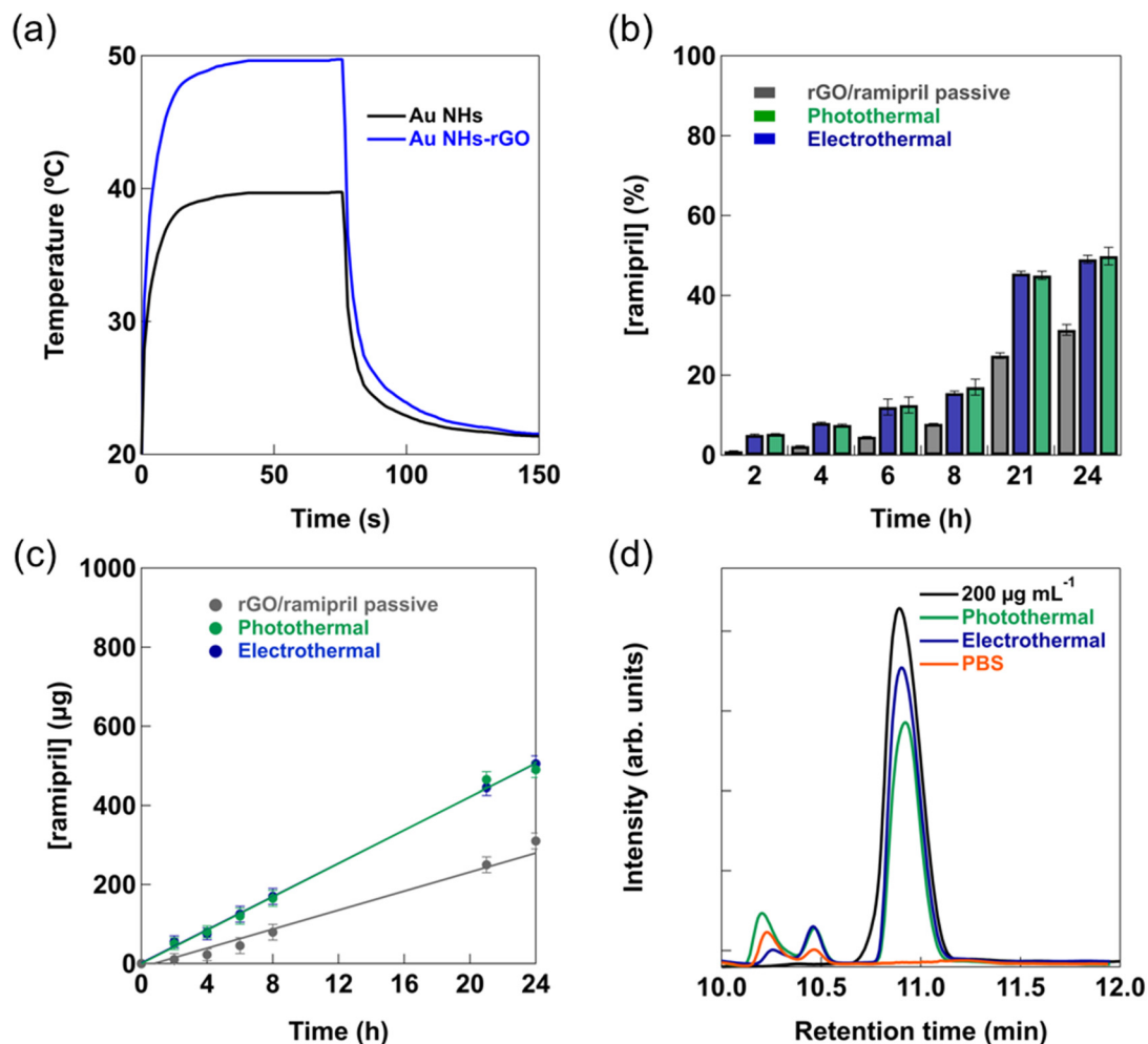
Fig. 3 Permeation of ramipril passively and under heat activation. (a) Temperature profiles over time upon the application of 1.0 V voltage bias on Au NHs and on Au NHs/-rGO bandages. (b) Ex vivo permeation profiles of rGO-nanoh heaters loaded with ramipril (1 mg in 1 mL of water) through rat skin either passively (black) or via photothermal (green) and electrothermal (blue) activation for 10 min ( n = 3 ). (c) Permeation profile of ramipril as a function of time. (d) HPLC profiles of ramipril ( 200 \mu\text{g mL}^{-1} ) before and after skin permeation under either photothermal ( 1 \text{ W cm}^{-2} ) or electrothermal (1.0 V) activation for 10 min. In a control experiment, PBS was permeated and the solution was analyzed. Error bars ( n = 3 ) represent standard error of the mean (SEM).
