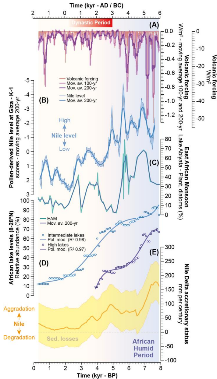
Fig. 3. Khufu-branch levels during the Holocene compared with volcanic forcing, East African Monsoon and North African lakes. (A) Volcanic forcing (58) expressed as Wm^{-2} and shown as events (red line), 100-yr (shaded light purple) and 200-yr (shaded dark purple) moving averages. (B) Pollen-derived Khufu-branch levels (K-1, blue line) expressed as 2.5 and 97.5 percentiles, and as a 200-yr moving average. (C) East African Monsoon (green line) reconstructed from planktonic diatoms recorded at Lake Abiyata - Ethiopia (24). The long-term trend is depicted by a 200-yr moving average (shaded blue line). (D) North African lake levels (blue: intermediate and purple: high lakes) (27) shown as relative abundances. Long-term trends are illustrated by polynomial models (order 3, P_{value} < 0.001 ). (E) Nile Delta accretionary status (20) shown in mm per century (orange) with the standard deviation (yellow). The background colors show the transition from the African Humid Period to the drying trend in Egypt.
