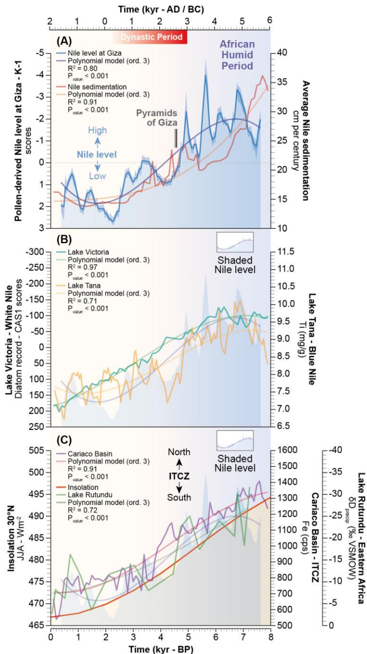
Fig. 2. Reconstructed Khufu-branch variations of the Nile during the last 8000 years. (A) Pollen-derived Khufu-branch levels (K-1, blue line) expressed as Loess smoothing scores (with 2.5 and 97.5 percentiles) compared with Nile Delta sedimentation rates (red line) (20). Long-term trends are depicted by polynomial models (order 3, P_{\text{value}} < 0.001 ). (B) Variations in Lake Victoria (White Nile) (23) and Lake Tana (Blue Nile) (22) reconstructed as a diatom record (red line) and Ti (mg/g; orange line). Long-term trends are depicted by polynomial models (order 3, P_{\text{value}} < 0.001 ). The Khufu branch is represented by a shaded curve. (C) Summer insolation (57), migration of the ITCZ (26) shown as \text{Wm}^{-2} (red line) and Fe (cps; purple line), and the Eastern African Monsoon shown as \delta D_{\text{precip}} (‰ VSMOW) (25). Long-term trends are denoted by polynomial models (order 3, P_{\text{value}} < 0.001 ). The Khufu branch is illustrated by a shaded curve. The background colors show the transition from the African Humid Period to the drying trend in Egypt.
