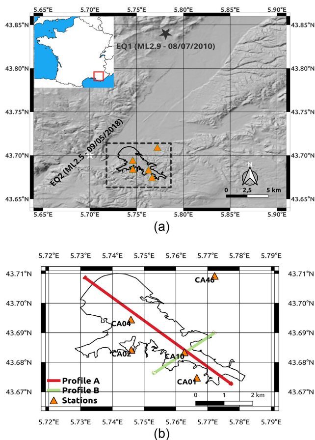
Figure 1. (a) Relief map of the surrounding areas around the Cadarache site. Orange triangles represent the available recording station. The elevation contour is expressed in meters above the mean sea level (MSL). The two small earthquakes recorded in the surroundings and indicated in Table 1 are reported [black (EQ1) and white (EQ2) stars, respectively]. The contour of the alluvial basin is indicated by the black line. (b) Detail of the sedimentary basin in the surrounding of the Cadarache area, including the recording stations available, employed by Perron et al. (2018) and the two cross-sections AA' and BB'.
