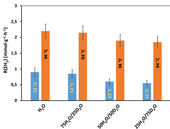
Fig. 2 Total hydrogen formation rate at different H_2O/D_2O ratios obtained at 52 and 94 °C. At other studied temperatures, a similar trend was observed.
