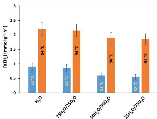
Fig. 2 Total hydrogen formation rate at different H_2O/D_2O ratios obtained at 52 and 94 °C. At other studied temperatures, a similar trend was observed.
