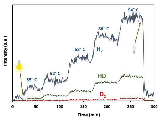
Fig. 1 Emission profiles of H_2 , HD, and D_2 species during photolysis of 50 mol.% H_2O/50 mol.% D_2O mixture in the presence of Ti@TiO_2 NPs and 1M glycerol irradiated with Xe-lamp under Ar-flow.
