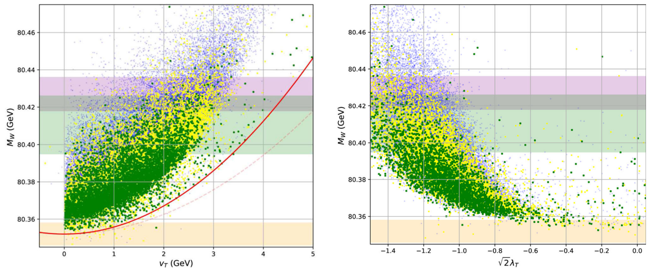
Fig. 5 W boson mass in the general DGNMSSM. Left: W boson mass against triplet expectation value. Right: W boson mass against \lambda_T . Colour coding of points as in previous figures
