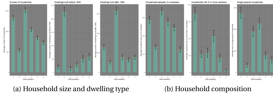
Figure 4: Error bars with confidence intervals showing the average grid parameter values after 1,000 draws (Heuristic).
