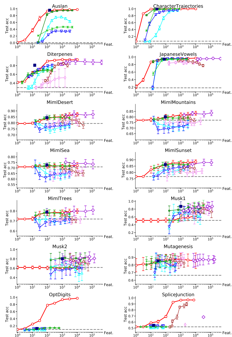
Fig. 10 Test accuracy versus original number of generated features per dataset.
