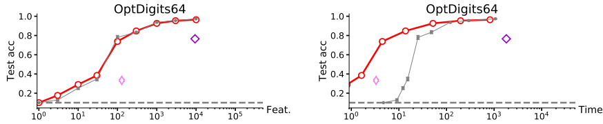
Fig. 13 Test accuracy result for the OptDigits dataset, using 4*4 blocks of pixels. MODL: ○ red MODL(pixel): ● gray Tilde: ◇ pink FORF: ◇ violet
