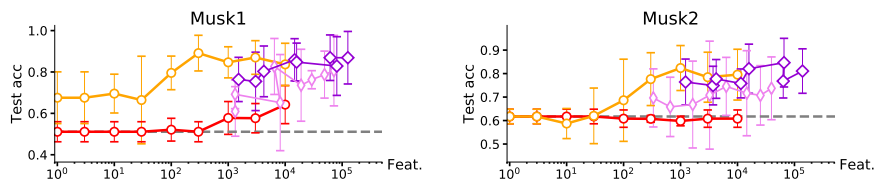
Fig. 14 Test accuracy result for the Musk1 en Musk2 datasets, with or without (NR) regularization of feature construction.
