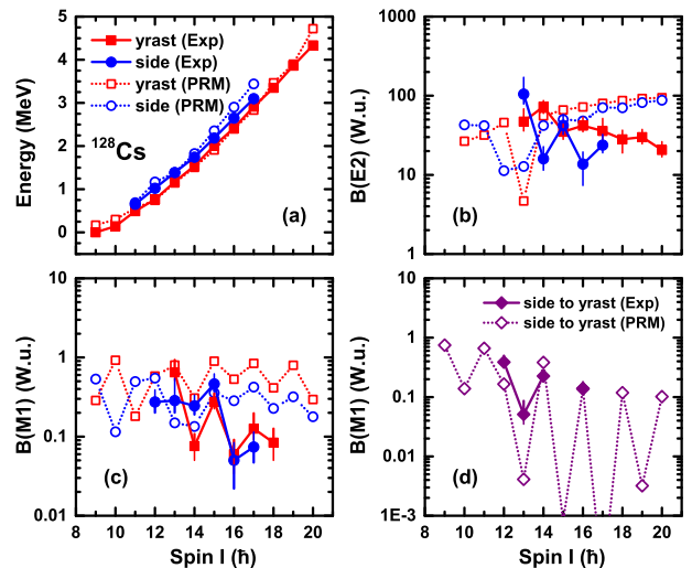
Figure 10: (a) The energy spectra, (b) the intradband B(E2) , (c) the intradband B(M1) , and (d) the interband B(M1) of the doublet bands in ^{128}\text{Cs} calculated by the PRM approach in comparison with the experimental data available [3].
