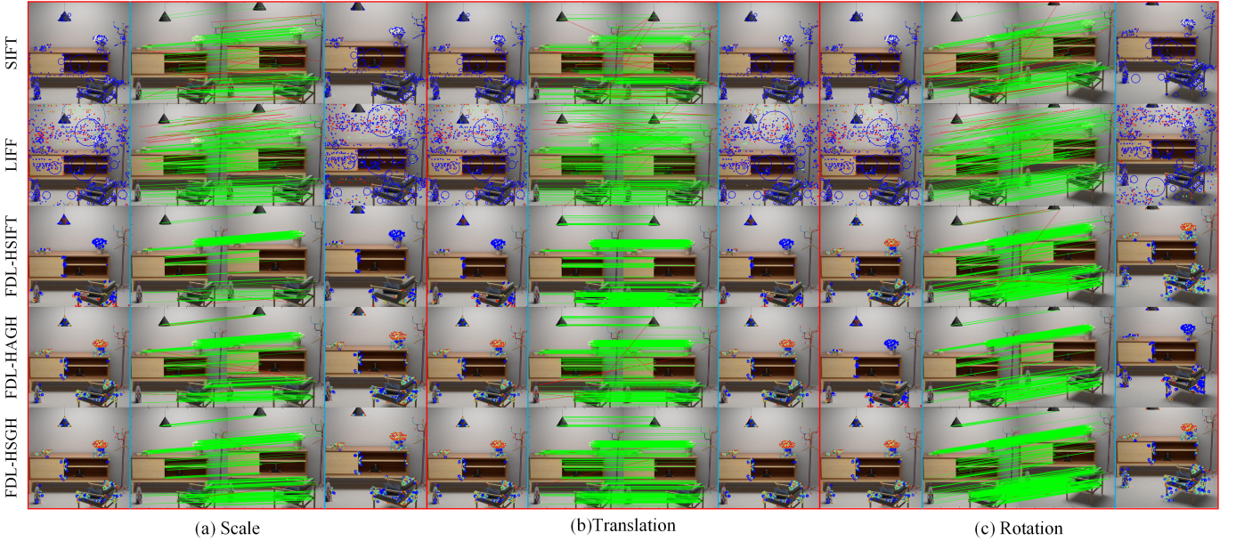
Fig. 12. Feature detection and matching results with synthetic LFs. (a) with scale transformation. (b) with translation. (c) with rotation.
