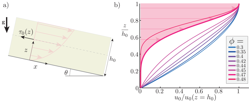
FIGURE 3. (a) Sketch of the notations. (b) Velocity profiles of the base flow for Wyart-Cates' rheology with the parameters obtained from figure 1b and for various volume fractions ( \tau_{b,0}/\tau^* = 2 ).
