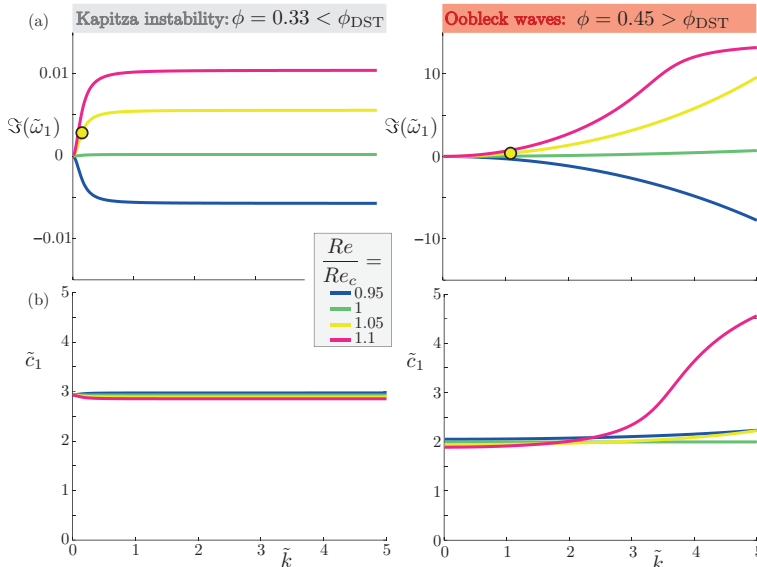
FIGURE 5. Dispersion relation of the two instabilities of the kinematic branch ( \theta = 10^\circ ). Left: Kapitza instability ( \phi = 0.33 ). Right: Oobleck waves instability ( \phi = 0.45 ). (a) Temporal growth rate \Im(\tilde{\omega}_1) . Note the highly different scales of the y-axis. (b) Wave speed \tilde{c}_1 . (a-b) The yellow circles indicate the theoretical growth rates, for Re = 1.05Re_c and at the wavelength observed experimentally, which are compared with measurements in figure 8b.
