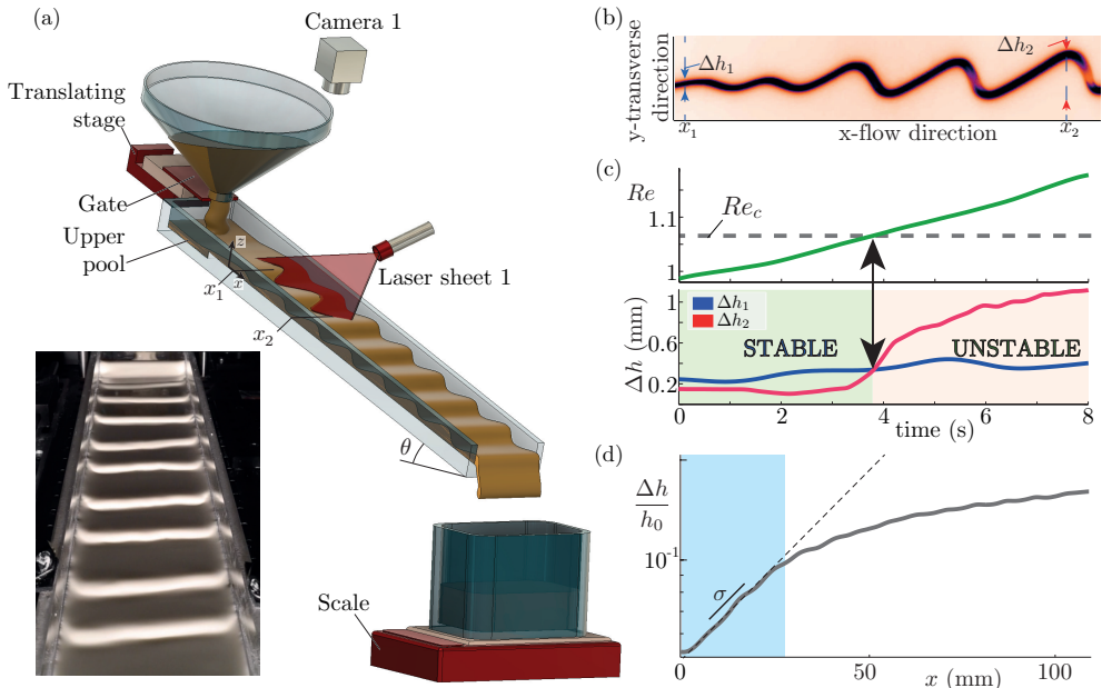
FIGURE 2. Experiments at high \phi to characterize the Oobleck waves. (a) Sketch of the set-up used for \phi > \phi_{\text{DST}} and typical image of Oobleck waves ( \phi = 0.45 , \theta = 10^\circ , Re \approx 1.14 \approx 0.2Re_{\text{Kap}} ). (b) Image of the flow surface intersected by the laser sheet (same condition as in (a)). (c) Reynolds number of the flow and amplitude of the perturbation \Delta h_1 and \Delta h_2 (same condition as in (a)). The black dashed line indicates the instability threshold Re_c . (e) Normalized wave amplitude \Delta h/h_0 as a function of x (same \phi and \theta , Re/Re_c = 1.05 ). The growth rate is measured over the region highlighted in blue.
