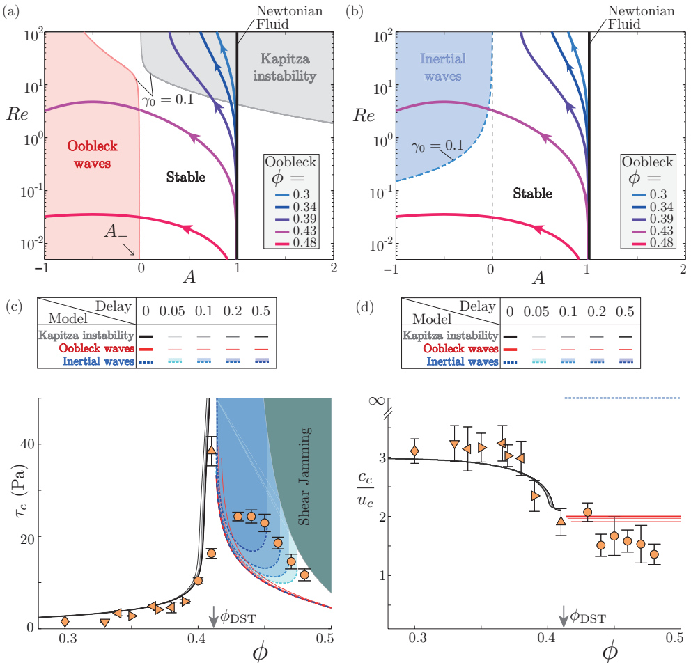
FIGURE 9. Role of a strain delay on stability. (a-b) Stability diagrams ( Re , A ) for the kinematic branch (a) and the inertial branch (b) ( \theta = 10^\circ , \alpha = 1 ). (a) The gray and red domains indicate the unstable regions for \gamma_0 = 0.1 . (b) The blue dashed line is the instability threshold (5.3) for \gamma_0 = 0.1 . The coloured lines indicate the system trajectories for increasing flow rate at fixed angle (same as in figure 4). The vertical dark lines indicates the Newtonian case ( A = 1 ). (c-d) Critical shear stress \tau_c (c) and normalized wave velocity c_c/u_c at the threshold (d) versus \phi . The symbols report the measurements presented in figures 7(b) and 8(c). The dark and red lines indicate the predictions for the kinematic branch below and above \phi_{DST} , respectively. The blue lines is the prediction for the inertial branch. The color intensity of the lines correspond to delay strains of \gamma_0 = 0.05, 0.1, 0.2 and 0.5 .
