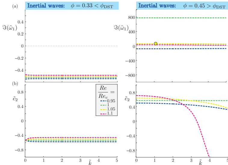
FIGURE 6. Dispersion relation of the inertial branch ( \theta = 10^\circ ). Left: \phi = 0.33 . Right: \phi = 0.45 . (a) Temporal growth rate \Im(\tilde{\omega}_1) . (b) Wave speed \tilde{c}_2 . The yellow circles indicate the theoretical growth rates, for Re = 1.05Re_c and at the wavelength observed experimentally, which are compared with measurements in figure 8b.
