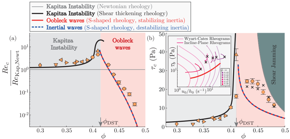
FIGURE 7. Destabilization threshold: comparison with experiments. (a) Critical Reynolds number Re_c normalized by the Newtonian Kapitza threshold Re_{Kap,Newt} = (5/6)/\tan\theta versus volume fraction \phi . (b) Critical basal shear stress \tau_c versus \phi . The symbols indicates measurements. Their shape encodes the inclination \theta : \diamond 2^\circ , \nabla 3^\circ , \triangleright 6^\circ , \triangleleft 9^\circ , \circ 10^\circ , \triangle 22^\circ . The error bars indicate the standard deviation of the measurements at a given \phi . The lines represent the predictions for the different modes (as labeled above the graph), i.e., the critical Reynolds number at which each iso- \phi trajectory (see figure 4) reaches the Re = Re_{Kap} or Re = Re_{A=0} condition (the black line is interrupted above \phi \simeq 0.42 since no steady flow verifies Re = Re_{Kap} ). The shear-jamming limit corresponds to the value of the basal shear stress when the flow first jams at z = 0 (see eq. 3.5). Inset: basal shear stress \tau_{b,0} = \rho gh_0 \sin\theta versus mean shear rate u_0/h_0 for different volume fractions obtained from Wyart-Cates rheological laws (dashed lines) and from direct measurements on the inclined plane (plain lines). The red line and black crosses highlight the condition d\tau_b/d\dot{\gamma} = 0 for both set of curves.
