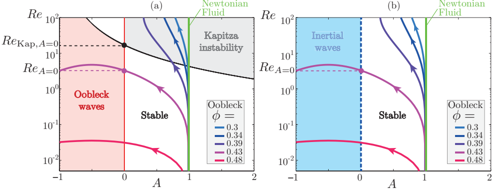
FIGURE 4. Stability diagram ( Re, A ) for (a) the kinematic branch and (b) the inertial branch ( \theta = 10^\circ and a plug flow profile ( \alpha = 1 ) is assumed for simplicity, see text). (a) Black line: Kapitza instability threshold ( Re = Re_{Kap} ). Red line: Oobleck waves instability threshold ( A = 0 ). (b) Dashed-blue line: inertial branch instability threshold ( A = 0 ). (a-b) The green line indicates the Newtonian case ( A = 1 ). The coloured trajectories indicate the evolution of Re and A for various volume fractions and increasing flow rates (or basal stress \tau_{b,0} ) ( \theta = 10^\circ and the rheological parameters are those obtained from figure 1b). For most volume fractions above \phi_{DST} , the discontinuous shear-thickening condition Re = Re_{A=0} (i.e., A = 0 ) is expected to be reached before (lower flow rate) the Kapitza instability onset ( Re = Re_{Kap} ).
