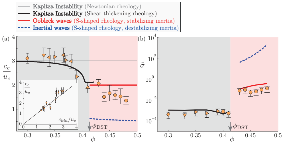
FIGURE 8. Wave speed and growth rate: comparison with experiments. (a) Wave speed c_c normalized by the mean fluid velocity u_c at the instability onset versus \phi . Inset: normalized wave velocity c_c/u_c versus normalized speed of kinematic waves c_{\text{kin}}/u_c at the onset. (b) Normalized spatial growth rate \tilde{\sigma} versus \phi for Re/Re_c = 1.05 .
