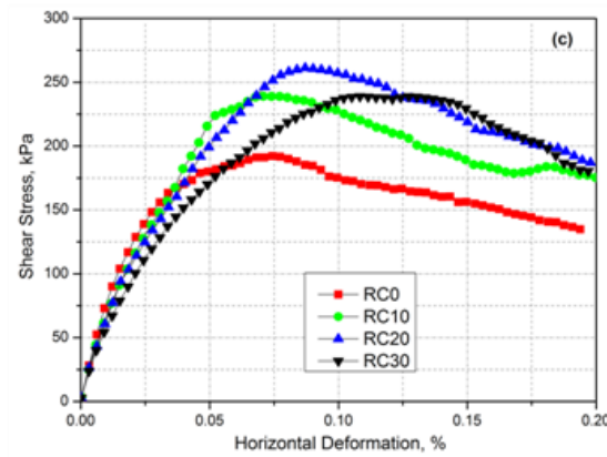
Figure 4. Shear stress variation curves for different rubber contents under a normal stress of: 100kPa (a), 200kPa (b) and 400 kPa (c) ( D_r = 55\% )
