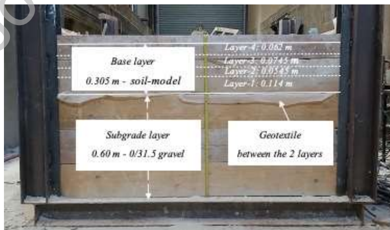
Figure 5: The different layers of the road platform
