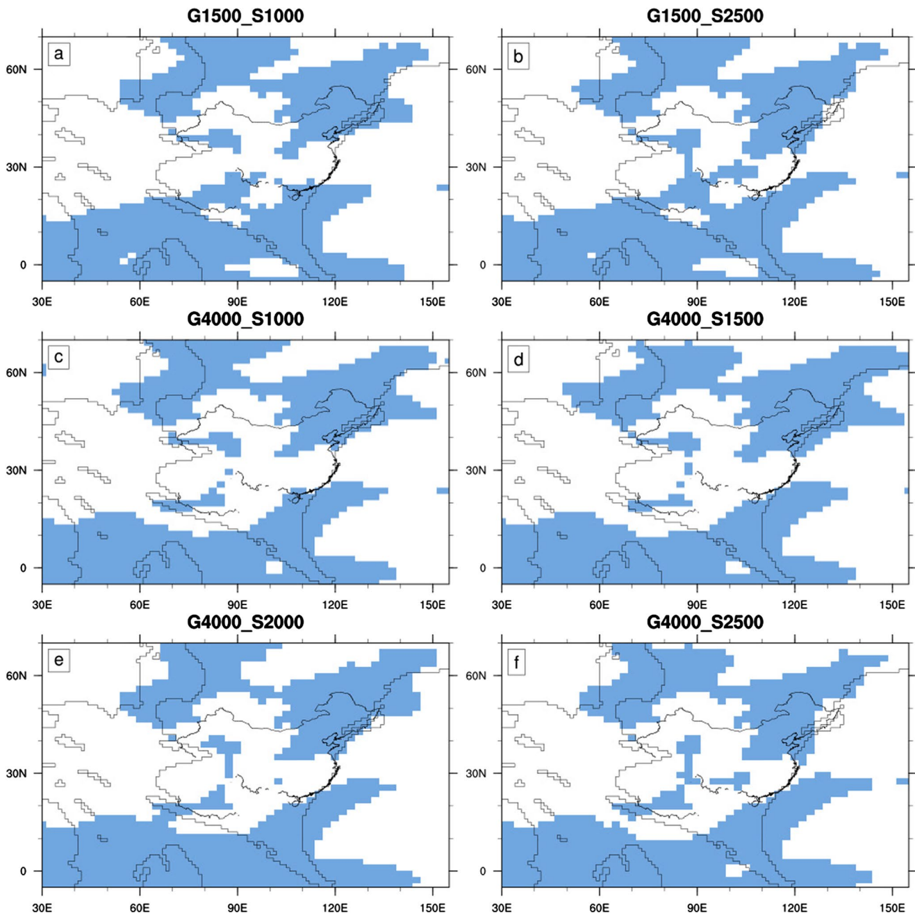
Figure 11. Monsoon domains defined by the SNS index (Li & Zeng, 2003). The shaded area shows SNS values >0. Sensitivity experiments are: (a) G1500_S1000, (b) G1500_S2500, (c) G4000_S1000, (d) G4000_S1500, (e) G4000_S2000, and (f) G4000_S2500.
