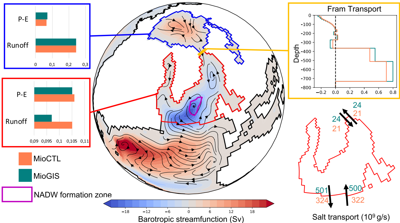
Figure 5. Mean annual barotropic streamfunction, in Sv, for the MioCTL simulation (in blue, the water masses rotate counterclockwise and in red, clockwise). The blue box shows the P-E balance and runoff (in Sv) for the Arctic basin. The red box shows the P-E balance and the runoff (in Sv) for the northern NA. The yellow box shows the water mass exchanges at the Fram Strait (in Sv), positive toward the north and negative toward the south. Bottom right, the salt transport budget (10 9 g/s). Values represent average on the last 100 years of each simulation.
