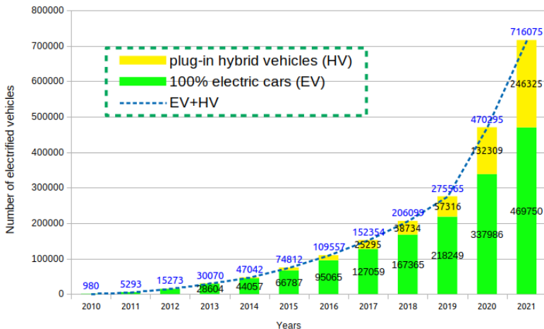
Fig. 1: Evolution of electric vehicle registrations in France.
