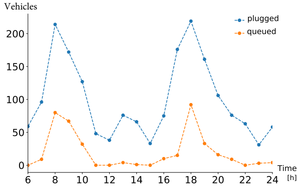
Fig. 10: Occupation of optimized 1 179 charging stations for 0.85% modal share.
