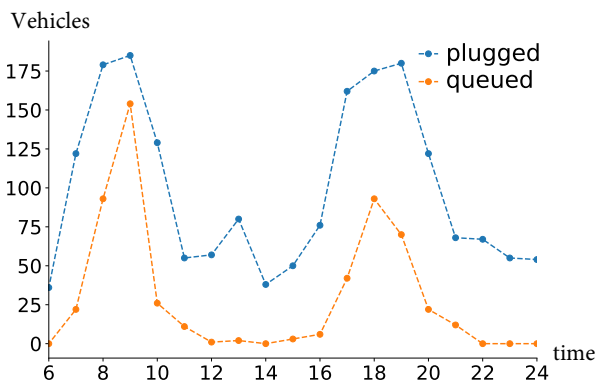
Fig. 9: Occupation of current 1 079 charging stations for 0.85% modal share.
