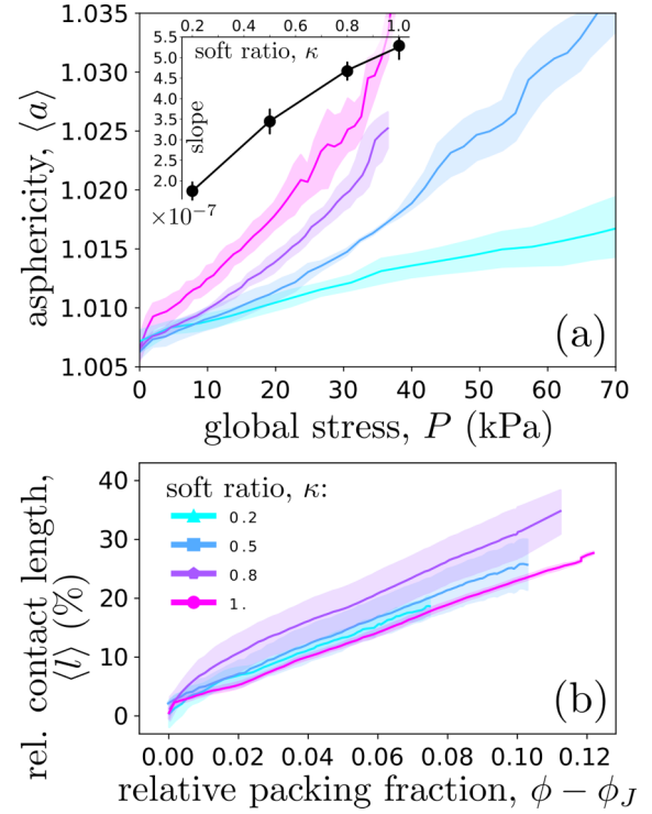
FIG. 3. (a) Linear evolution of the soft particle average asphericity \langle a \rangle as a function of the global stress applied to the system P . Their slope is given in the inset as a function of the softness ratio \kappa . (b) Linear evolution of the average value of the relative contact length \langle l \rangle as a function of the distance to the jamming transition for the packing fraction \phi - \phi_J . In both panels, the different curves correspond to different \kappa , given in the legend in (b).
