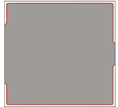
FIGURE 5 Density \rho = 0.5 of the initialization structure for the cantilever test case (the boundary of \Omega is the red line)
