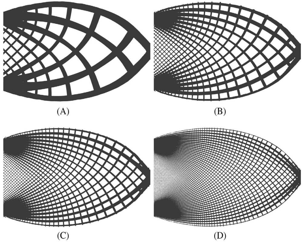
FIGURE 8 Projected structures \Omega_\varepsilon(\varphi, m) for several \varepsilon in the case of the cantilever, with m_{\max} = 0.8 . A, \varepsilon = 0.4 . B, \varepsilon = 0.2 . C, \varepsilon = 0.1 . D, \varepsilon = 0.05
