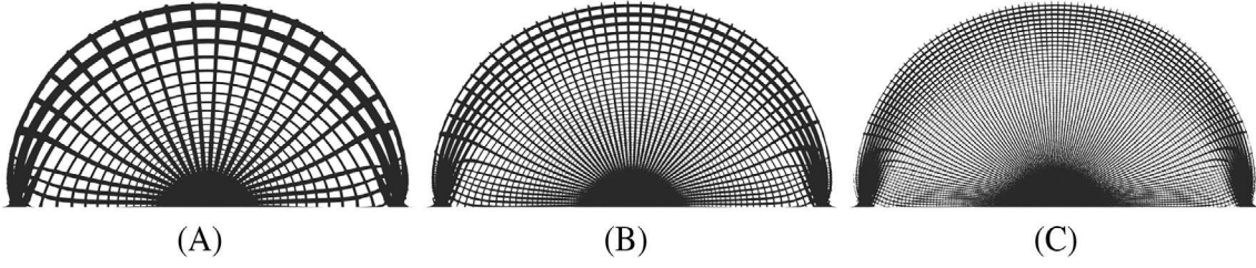
FIGURE 11 Projected structures \Omega_\varepsilon(\varphi, m) for several \varepsilon in the case of the bridge. A, \varepsilon = 0.2 . B, \varepsilon = 0.1 . C, \varepsilon = 0.05
