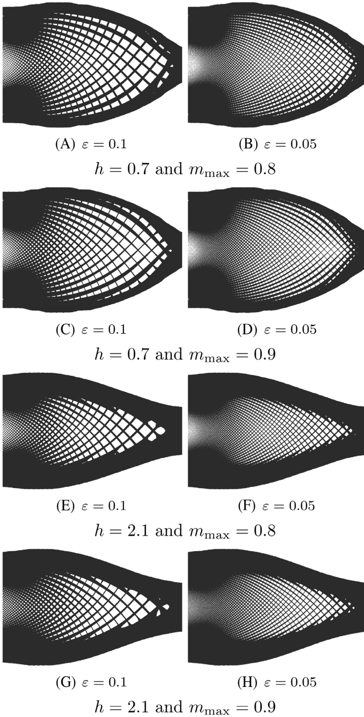
FIGURE 13 Projected structures \Omega_\varepsilon(\varphi, m) for several \varepsilon in the case of the coated cantilever. A, \varepsilon = 0.1 . B, \varepsilon = 0.05 . C, \varepsilon = 0.1 . D, \varepsilon = 0.05 . E, \varepsilon = 0.1 . F, \varepsilon = 0.05 . G, \varepsilon = 0.1 . H, \varepsilon = 0.05
