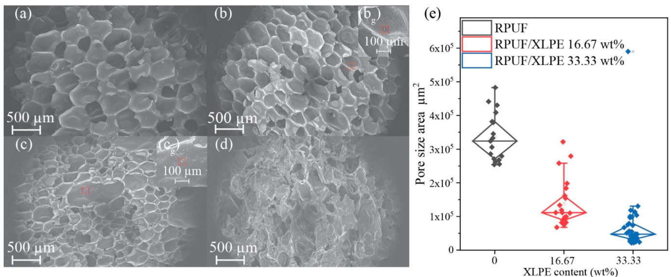
Figure 5. The SEM images for foams of the (a) RPUF, (b) RPUF/XLPE 16.67 wt%, (b g ) XLPE microparticle fillers with 100 µm scalebar, (c) RPUF/XLPE 33.33 wt%, (c g ) XLPE microparticles, and (d) RPUF/XLPE 47.37 wt%, (e) whisker box plot of pore size area vs. XLPE content.
