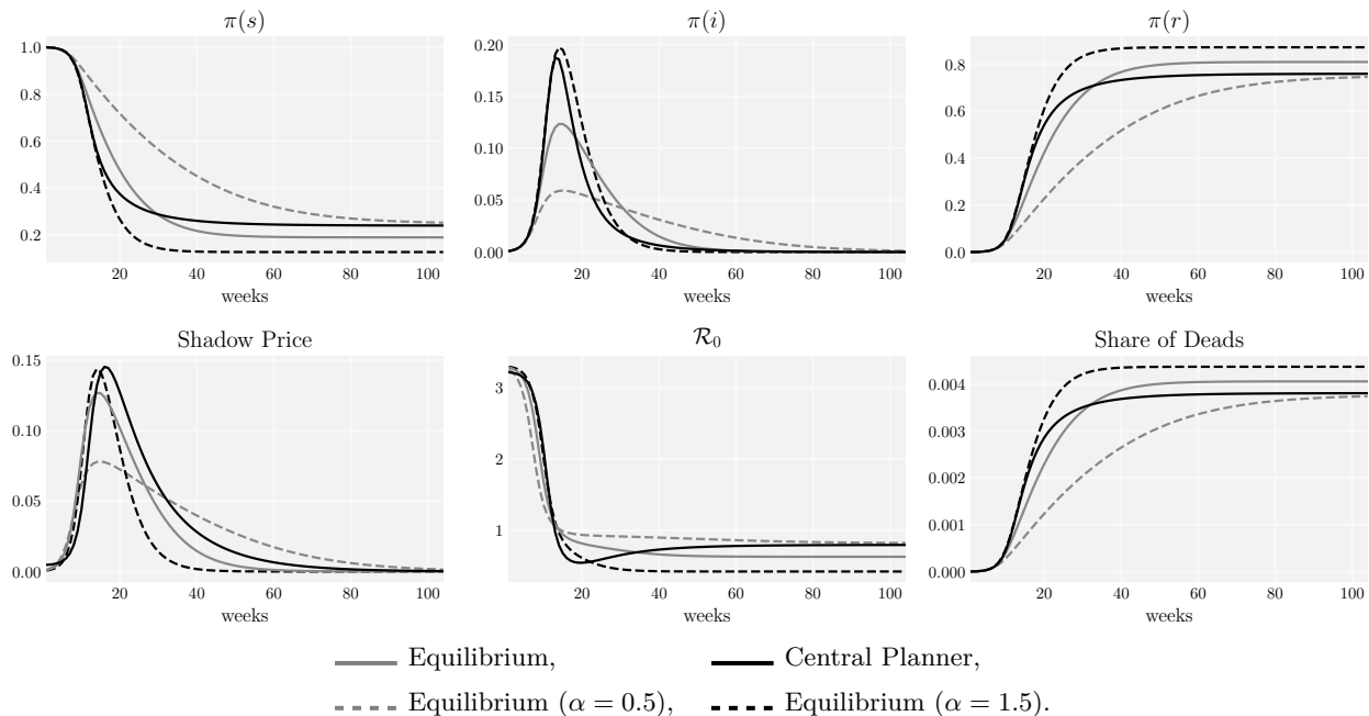
Figure 9: Varying \alpha
