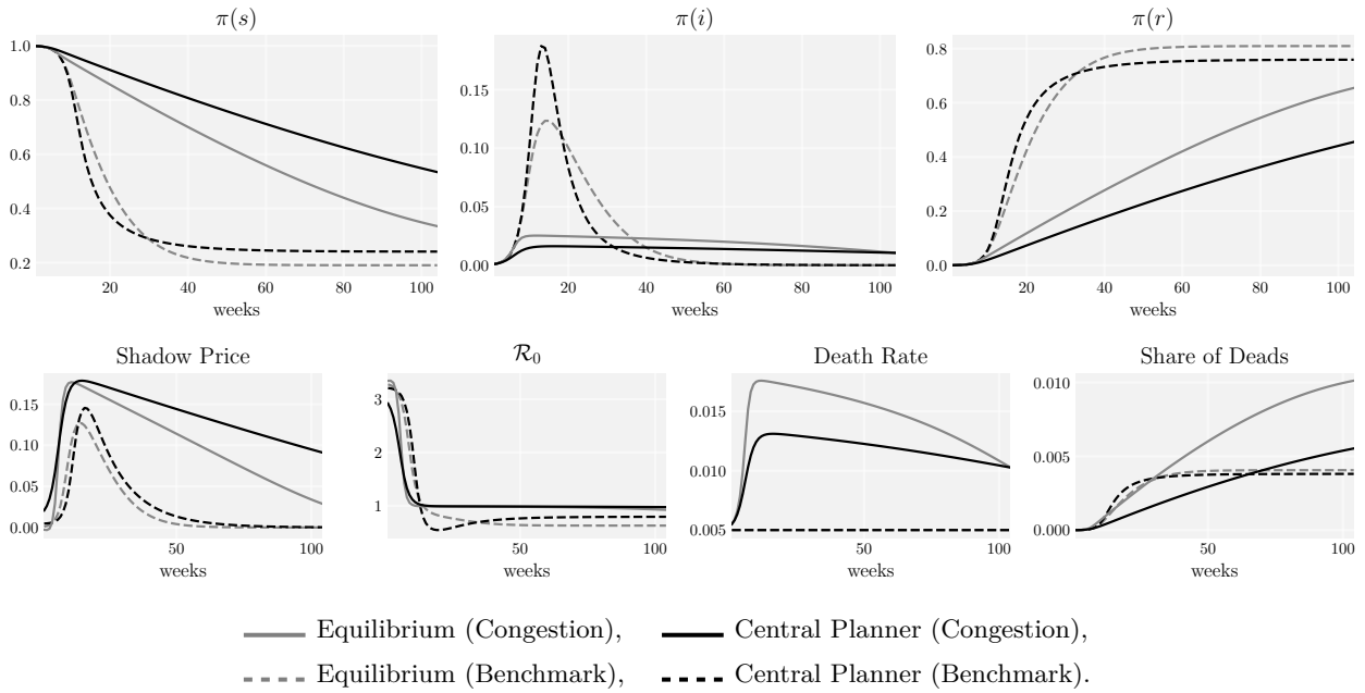
Figure 10: Congestion Effects
