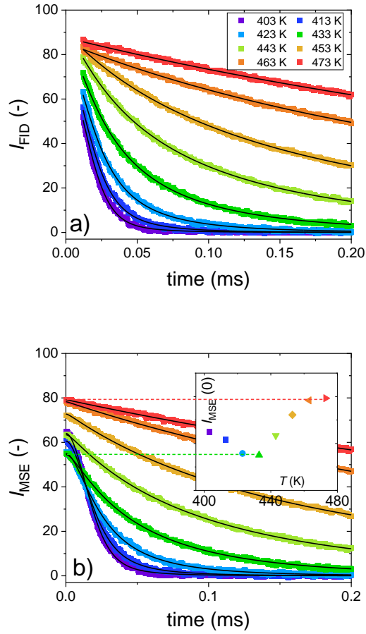
Figure 3: a) Raw I_{FID}(t) signal measured from the neat P2VP between 403 and 473 K. b) Analogous data for I_{MSE}(t) . Solid lines represent joint fits to the data (I_{FID}, I_{MSE}) for each temperature with the AW function (Equation 3) considering a log-normal distribution of \tau_c (see text). The inset shows the expected non-monotonic variation of the MSE-FID signal at short time with the temperature (see refs. 19,20 ).
