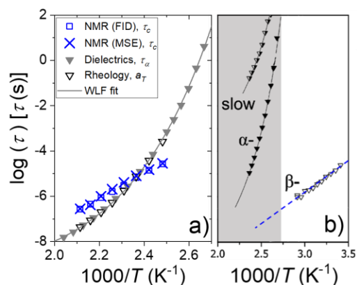
Figure 4: Temperature dependence of the neat P2VP segmental relaxation time. Panel a) shows data from our previous publication probed by dielectric spectroscopy ( \tau_\alpha ) and rheology ( a_T ), 9 together with the low-field NMR ( \tau_c ). The solid line is a fit of the dielectric data based on the WLF model at a reference temperature of 373 K. Panel b) shows dielectric data for a high molecular weight P2VP ( \overline{M}_n \sim 30 \text{ kDa} ) adapted from ref. 29 – see details in the text, with the grey shaded region indicating the temperature range in a).
