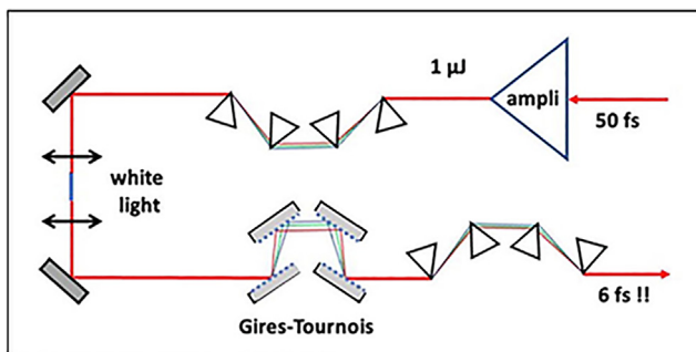
FIG. 1.11 – Designs of a very short optical pulse generator. 50 \text{ fs} amplified pulses with an energy of 1 \mu\text{J} are first set to their Fourier transform limit through a prism optical compressor. Producing pulses 10 times shorter means widening the light spectrum by the same amount; this is achieved by self-phase modulation inside a short single-mode optical fiber 1 \text{ cm} long. The resulting white light pulse is then recompressed to third-order dispersion via a grating + double prism optical compressor resulting in ultra-short light pulses of 6 \text{ fs} .
