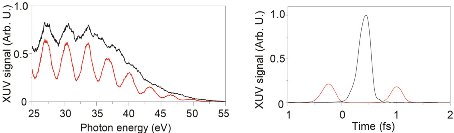
FIG. 6.17 – Effect of a change of the CEP on the spectrum (left panel) and corresponding temporal profile (right panel) for an attosecond source driven by a polarization gate field (from 23 ).
