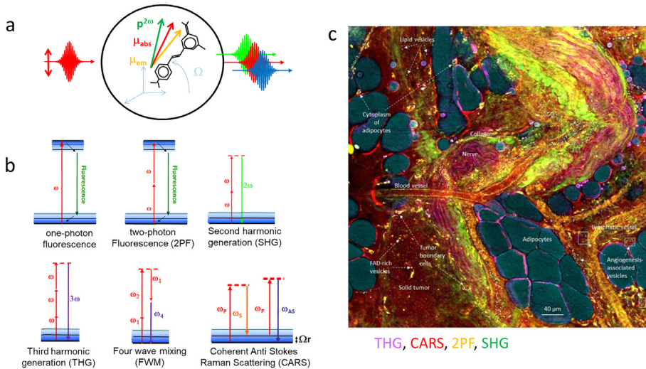
FIG. 9.1 – (a) Schematic drawing of a molecule excited by different frequencies. The radiation from the molecule originates either from an emission transition dipole moment (fluorescence), or from a nonlinear induced dipole moment (coherent second-order nonlinear optical process). (b) Energy diagram scheme of the different contrasts addressed in this lecture: one- and two-photon excited fluorescence (2PF) and the nonlinear coherent processes SHG, FWM, THG, and CARS. (c) Co-registered multi-modality image of a mammary tumor from a carcinogen-injected rat. The image ( 1140 \times 1140 pixels with 0.5 \mu\text{m} pixel size) was collected by label-free nonlinear microscopy with multiple pseudo-colour contrasts: magenta-THG; red-CARS (lipids); yellow-2PF; green-SHG. Various structures in the tumour microenvironment are visible. From 10 .
