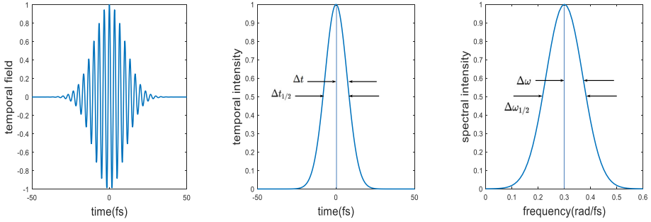
FIG. 2.2 – Temporal field, temporal and spectral intensities of a Gaussian pulse.
