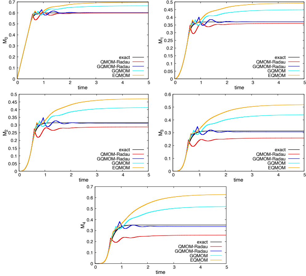
Figure 10: Test case with nucleation, growth and filtration: moments of order 0, 1, 2, 3 and 4 for the analytical solution, QMOM–Radau with five moments (i.e., \mathbf{M}_4 ), gamma–GQMOM and gamma–GQMOM–Radau with five moments and N = 20 and gamma–EQMOM with 10 secondary quadrature points.
