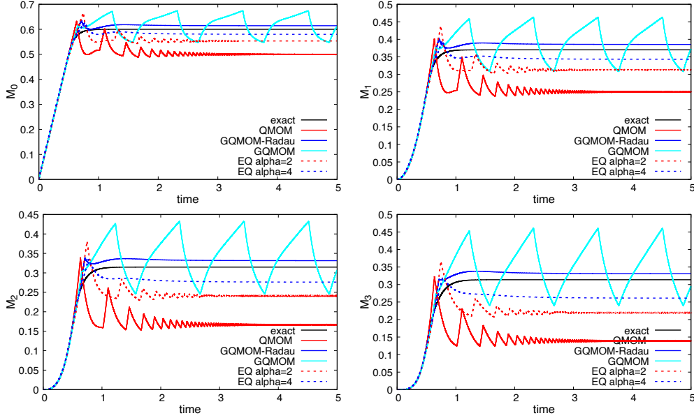
Figure 11: Test case with nucleation, growth and filtration: moments of order 0, 1, 2 and 3 for the analytical solution, QMOM with four moments (i.e., \mathbf{M}_3 ), gamma-GQMOM and gamma-GQMOM-Radau with four moments and entropic quadrature (EQ) with multiplicative factor \alpha = 2 and \alpha = 4 .
