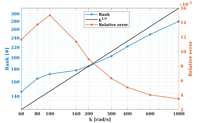
Fig. 5: Accuracy of the solution and rank of the compressed matrix as a function of k , with a compression parameter \epsilon = 0.015 .
