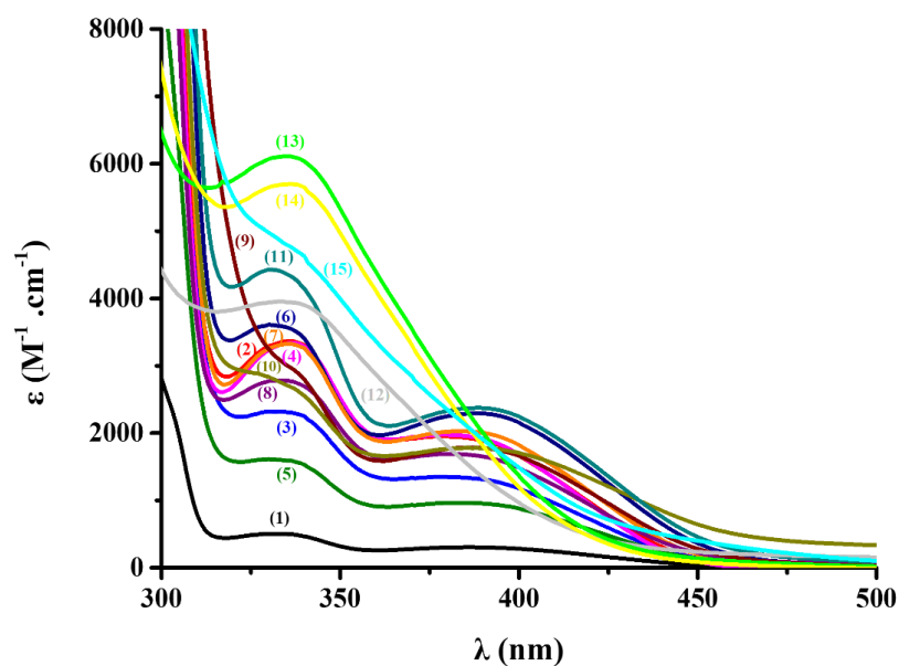
Figure 1. UV-Visible Absorption properties of 1-15 in acetonitrile.
