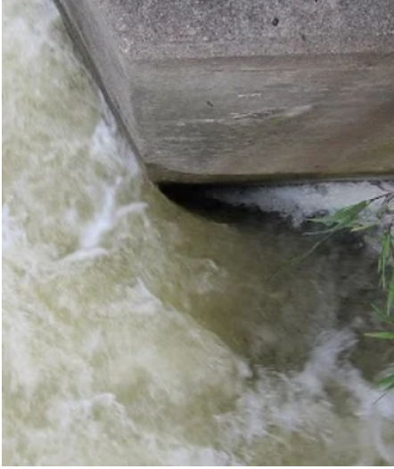
Figure 11: Illustration of the Vena Contracta phenomenon. Source: Meholic (2018).
