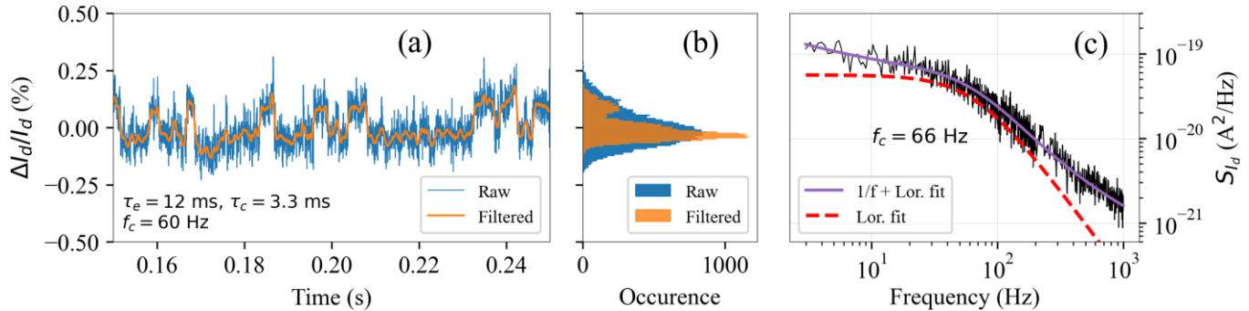
Figure 7: (a) Noise measurement before (blue lines) and after filtering (orange lines). (b) Associated histograms. (c) Noise spectrum of the raw signal fitted with the hybrid Lorentzian- 1/f^\alpha model (purple line) and the Lorentzian model (red dashed line).
