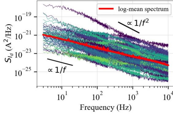
Figure 1: Measurement example of drain current noise spectra for 59 n-MOS transistors and the associated 1/f log-mean spectrum (red line).
