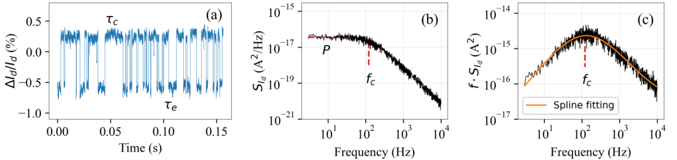
Figure 2: (a) Time domain measurement exhibiting RTN. (b) Associated Lorentzian spectrum with cut-off frequency f_c and plateau P . (c) Spectrum multiplied by the frequency.
