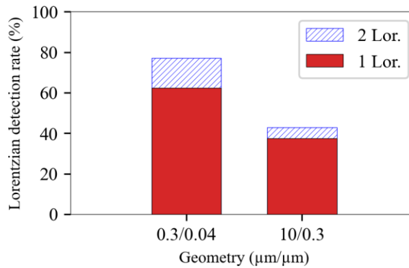
Figure 4: Average detection rates of the presence of Lorentzians in n-MOS transistors of geometries W = 0.3 \mu\text{m} , L = 40 \text{ nm} and W = 10 \mu\text{m} , L = 0.3 \mu\text{m}
