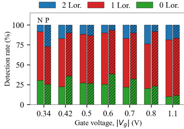
Figure 3: Detection rates of the presence of Lorentzians in the noise spectra of 59 n-MOS (left bars) and p-MOS (right hashed bars) transistors of geometry W = 0.3 \mu\text{m} , L = 40 \text{ nm} for different gate voltages |V_g| .
