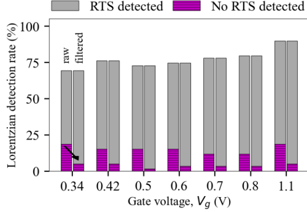
Figure 5: Detection rates of the presence of RTS within the 59 n-MOS spectra showing Lorentzians before (left bars) and after time-domain filtering (right bars) for different gate voltages V_g .
