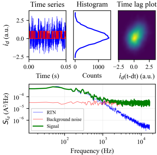
Figure 6: Simulation example of RTS hidden behind a background noise such as its histogram and time-lag plot show no significant RTS trace. The processed spectrum still shows a Lorentzian followed by the constant PSD of the background white noise ( C in equation (2)).
