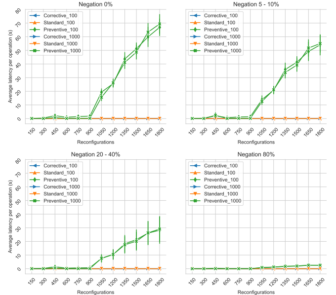
Fig. 9. Latency per reconfiguration operation, lower is better. Both the corrective and standard algorithms are instantaneous, while the preventive variant must wait. For 1800 concurrent reconfigurations the average latency per operation is 1 minute for preventive variant.
