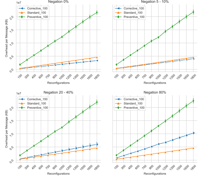
Fig. 11. Overhead per messages, lower is better. Delay and negation seem to not impact the preventive and the standard algorithms. For the corrective variant, negation has the greatest impact since more data is sent every time a negation happens.
