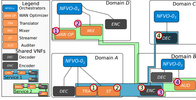
Fig. 1. Example of composite services with shared VNF-FGs. Four administrative domain have composite services that use shared VNFs and their replicas. This creates dependencies in the VNF-FGs.
