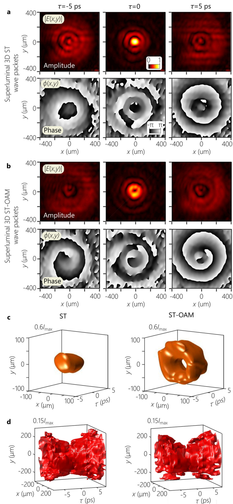
Fig. 7 | Measured complex-field amplitude and phase profiles for 3D ST wave packets with and without OAM. a Measured amplitude |E(x,y)| (first row) and phase \phi(x,y) (second row) at a fixed axial plane z = 30 mm (see Figs. 5 and 6) at delays \tau = -5 ps, \tau = 0 corresponding to the wave-packet center, and \tau = 5 ps for a
