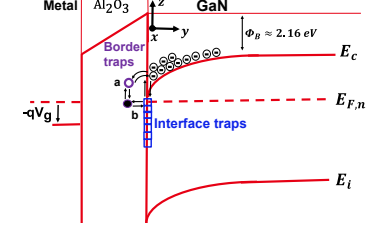
Fig. 17: Energy band diagram showing the tunnelling mechanism of electrons between the conduction band
