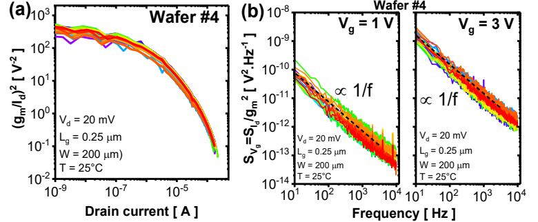
Fig. 9: (a) (g_m/I_d)^2 characteristics with logarithmic scale and (b) Input-referred gate voltage noise S_{id}/g_m^2 versus frequency for 25 devices with L_g=0.25 \mu m at two different biases (1V and 3V)
