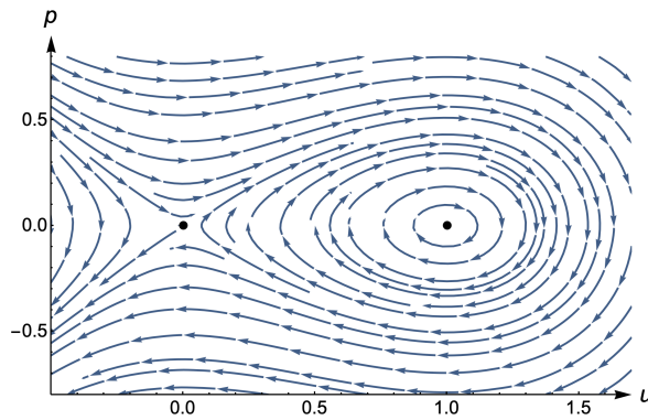
Figure 4: The phase portrait for the system (19). The relaxation parameter is set to \tau = 0.001 whereas a dispersion parameter is chosed \varepsilon = 0.75 and the velocity of the solitary wave is s = 0.5 . The homoclinic orbit in the phase plane starting and ending in (0, 0) saddle point corresponds to a solitary traveling wave solution.
