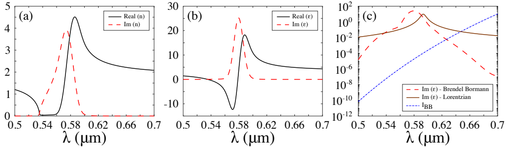
Fig. 5. (a) The complex refractive index n of TDBC obtained with a Brendel-Bormann model, (b) the complex dielectric permittivity \epsilon of TDBC and (c) the imaginary part of the complex dielectric permittivity of TDBC obtained with a Brendel-Bormann model (red dashed line) or with a Lorentzian model (brown plain line) compared to the Planck function I_{BB} (blue dotted line).
