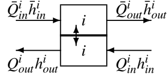
Figure 1: Elementary block i with enthalpy flows
