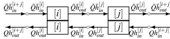
Figure 2: Two heat exchangers or two heat exchanger networks in series
