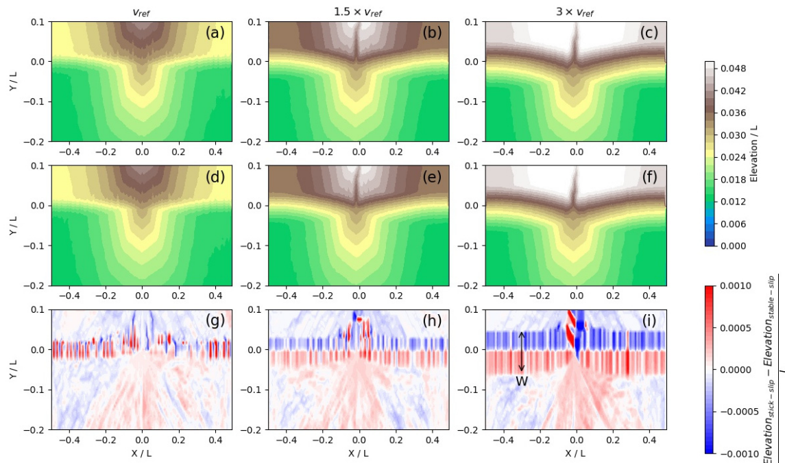
Figure 11. Morphological signature of fault slip rate. (a) Elevation associated with stick-slip behavior assuming the fault slip rate v_{ref} used in the numerical reference model (see Table 1). (b,c) same as (a), assuming a fault slip rate of 1.5 \times v_{ref} and 3 \times v_{ref} , respectively. (d–f) same as (a–c), assuming a stable sliding. (g–i) elevation deviation between slick-slip and stable sliding for a fault slip rate of v_{ref} , 1.5 \times v_{ref} , and 3 \times v_{ref} , respectively. W is the width of the zone with a high elevation deviation.
