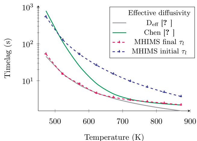
Figure 13: Comparison of the timelags evaluated using equation (21) with several effective diffusivities, assuming a sample thickness of 500 \mu\text{m} . At higher temperatures, the effect of the irreversible trap vanishes and all plots show a similar trend; however, at lower temperatures, the first timelag and the timelag evaluated using [?] are up to an order of magnitude higher than other timelags.
