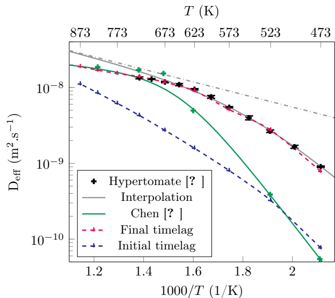
Figure 12: Comparison of the initial vs. steady-state timelag on effective diffusivity, using the adjusted densities model. The interpolation law and experimental points given in [?], corrected in order to be compared with hydrogen results are shown. The dashdotted line represents interstitial diffusivity D introduced in equation (3).
