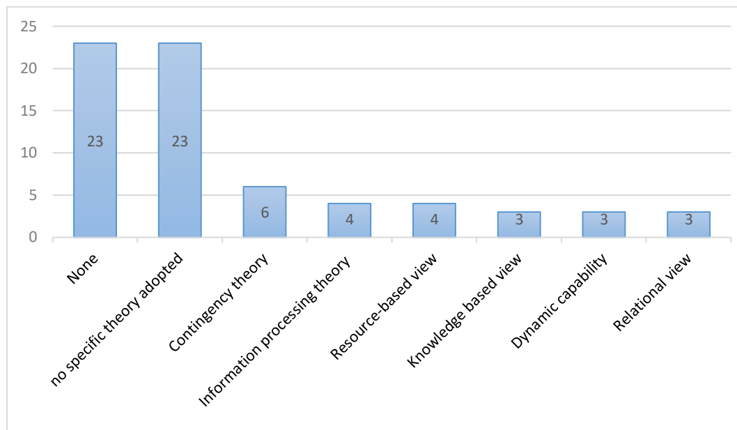
Figure 4 – Theories used
