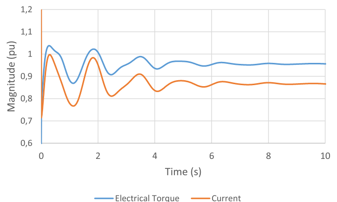
Fig. 6. Evolution of the electrical torque and the current of generator 3 after a short-circuit.
