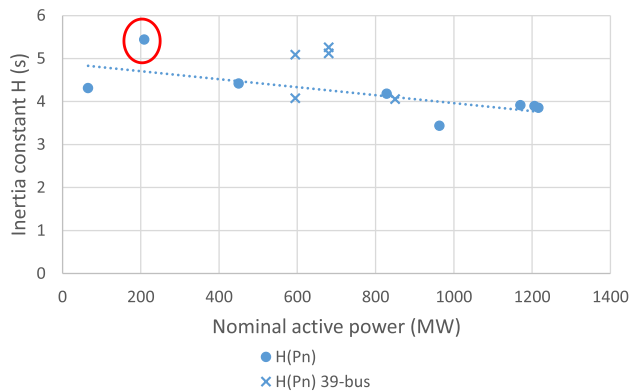
Fig. 9. Evolution of nuclear unit's inertia constants as a function of nominal active power in the 39-bus grid and according to [19].
