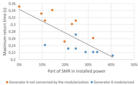
Fig. 16. Evolution of maximum return time against the part of modularized installed capacity in the grid.
