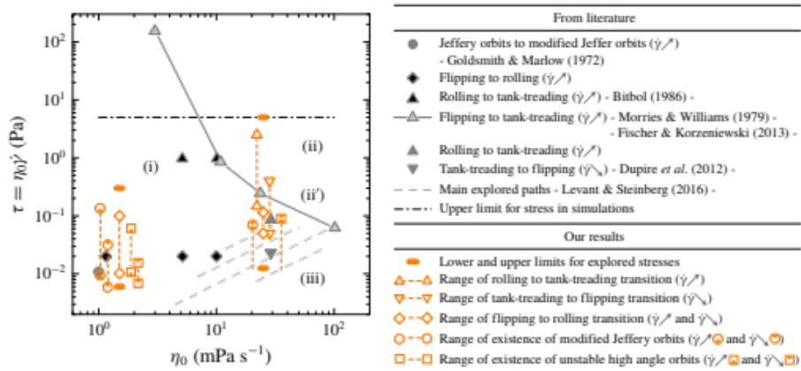
Figure 1.4. Transitions between dynamic regimes of the shear red blood cell identified in the literature and transition ranges observed on a large sample of red blood cells (Minetti et al. 2019).
