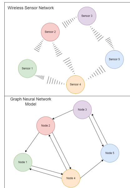
Fig. 1. Modeling a sensor network into a directed Graph Neural Network
