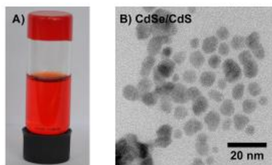
Figure 1. a) Image of an upside down vial containing wurtzite CdSe QDs synthesized with the method described in the literature, 23 with the solidified fraction still attached to the bottom of the vial. b) TEM image of core-shell QDs grown from the solidified CdSe cores which result in particles with poor structural morphology.
