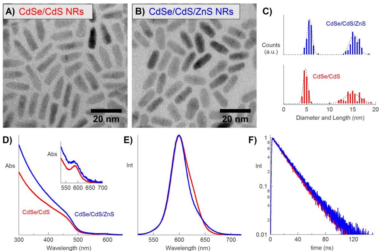
Figure 8. TEM images of a) CdSe/CdS and b) CdSe/CdS/ZnS NRs with c) histograms of the diameters and lengths measured from TEM images. Optical properties with d) absorption spectra normalized to QD concentration determined by ICP measurements (inset: focus on the excitonic feature at 590 nm), e) normalized emission spectra and f) normalized photoluminescence decays of the NRs.
