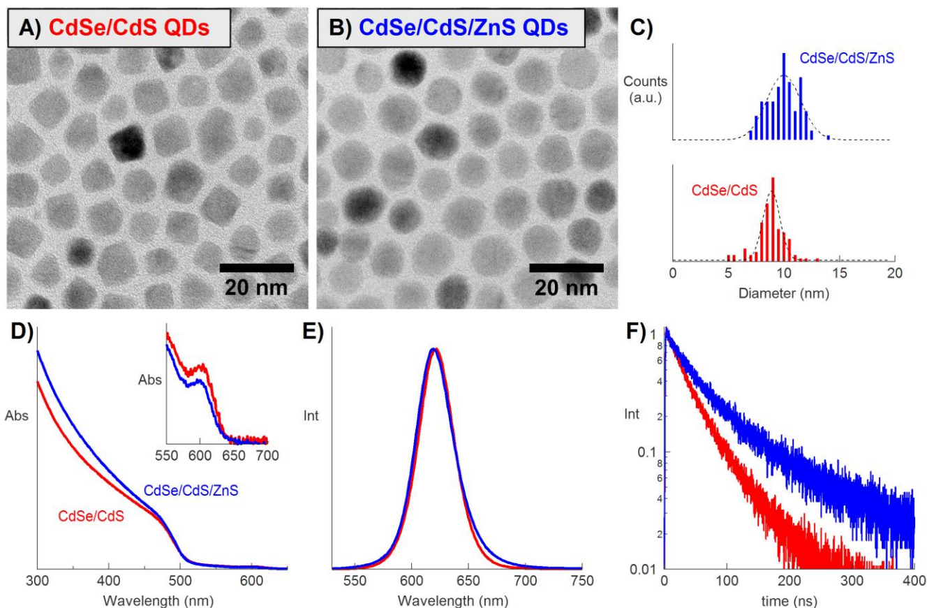
Figure 4. TEM images of a) CdSe/CdS and b) CdSe/CdS/ZnS QDs with c) histograms of the diameters measured from TEM images. Optical properties with d) absorption spectra normalized to QD concentration determined by ICP measurements (inset: focus on the excitonic feature at 600 nm), e) normalized emission spectra and f) normalized photoluminescence decays of the QDs.
