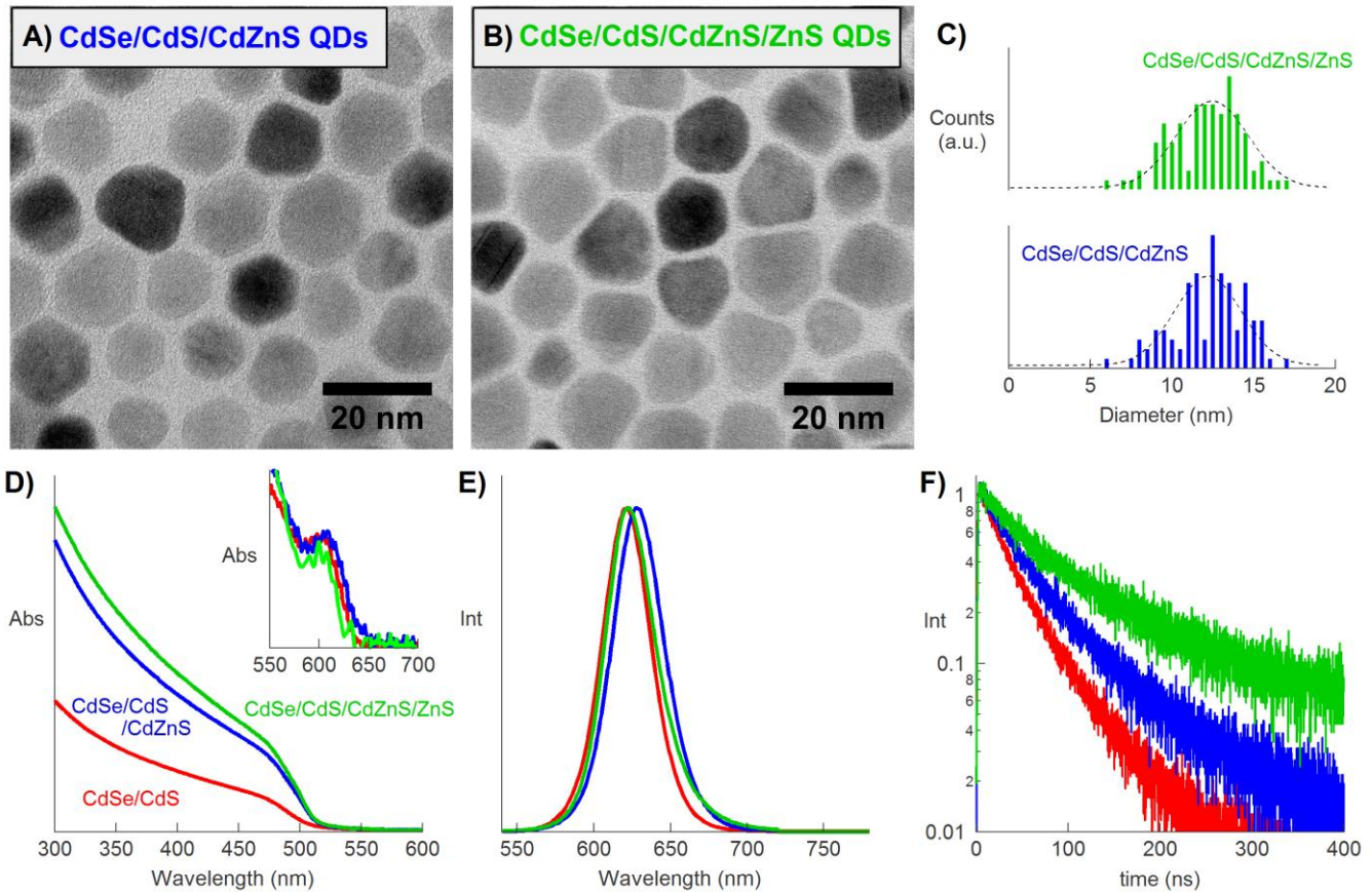
Figure 6. TEM images of a) CdSe/CdS/CdZnS and b) CdSe/CdS/CdZnS/ZnS QDs with c) histograms of the diameters measured from TEM images. Optical properties with d) absorption spectra normalized to QD concentration determined by ICP measurements (inset: focus on the excitonic feature at 600 nm), e) normalized emission spectra and f) normalized photoluminescence decays of the QDs.
