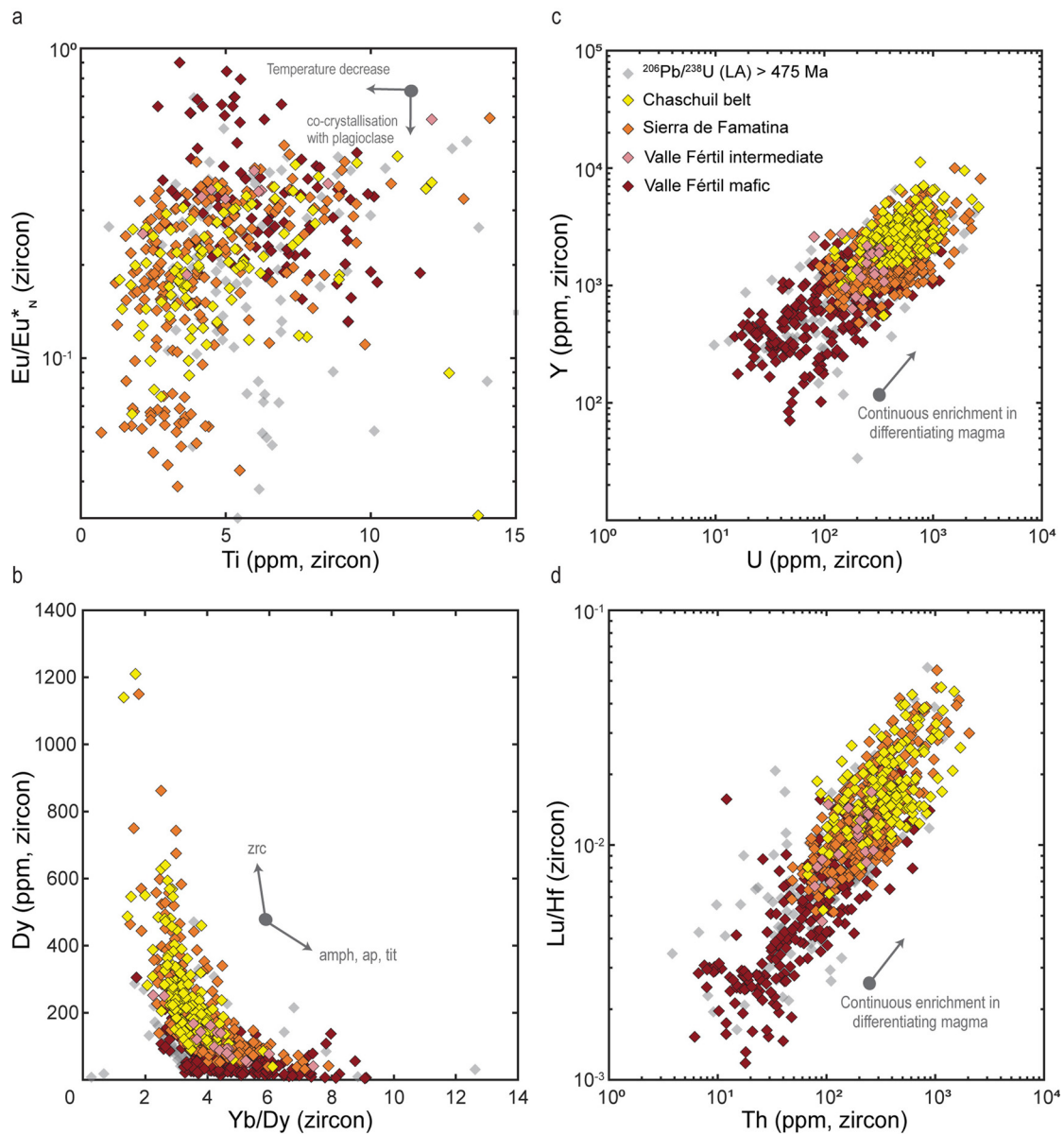
Fig. 3. Zircon trace element geochemistry of the Famatinian plutonic arc samples along the N-S transect excluding the peripheral units. (a) \text{Eu}/\text{Eu}_N^* vs. Ti highlighting the effect of plagioclase accumulation in a cooling magma prior to zircon saturation. \text{Eu}/\text{Eu}_N^* normalized to the depleted mantle (Salters and Stracke, 2004), (b) Dy vs. Yb/Dy shows the evolution of mid-Rare Earth (MREE) against Heavy-REE (HREE) and the control of zircon upon the REE budget as the melt temperature decreases and composition evolves towards more silicic. (c) and (d), displaying linear trends of Y vs. U and Lu/Hf vs. Th respectively, show the dominating control of zircon on the budget of these elements and the increase of zircon/melt partition coefficients owing to decreasing temperature and evolving melt composition towards more silicic.
