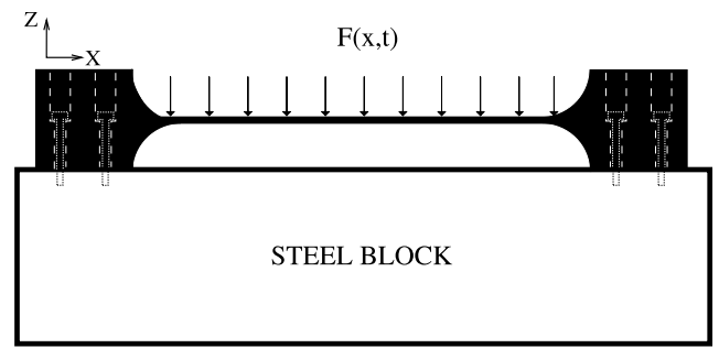
Fig. 1. A diagram of the non-ideal clamped-clamped CEA-beam structure solicited by N_e punctual correlated temporal forces.
