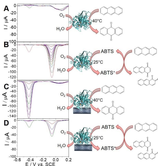
Figure 3. (A) SWV (0.1 M McIlvaine buffer pH 5, 25°C, pulse height = 25 mV, pulse width = 0.5 s, step height = -5 mV) for the detection of different concentrations of anthracene (0, 0.1 nM, 100 nM, 1 μM and 100 μM) after incubation (10 min) of the MWCNT electrode in a solution of 1 U mL -1 of laccase and anthracene left to react for 2 h at 40 °C min ; (B) SWV for the detection of different concentrations of anthracene (0, 0.1 nM, 10 nM, 0.1 μM, 1 μM, 10 μM and 100 μM) after incubation (10 min) of the MWCNT electrode in a solution of 1 U mL -1 of laccase and ABTS left to react for 1 h at 25 °C min ; (C) SWV for the detection of different concentrations of anthracene (0, 0.1 nM, 10 nM, 0.1 μM, 1 μM, 10 μM and 100 μM) after incubation (10 min) of a POXA1b modified electrode in a solution of anthracene left to react for 2 h at 40 °C ; (D) SWV for the detection of different concentrations of anthracene after incubation (10 min) of a POXA1b-modified electrode in a solution of anthracene (0, 0.1 nM, 100 nM, 1 μM and 100 μM) and ABTS left to react for 1 h at 25 °C
