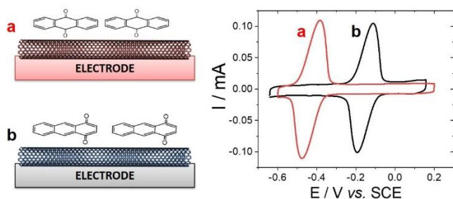
Figure 1. 3D Schematic representation of adsorbed 1-9 anthraquinone and 1,4 anthraquinone at MWCNT electrode and CV of the modified MWCNT electrodes performed in 0.1 M McIlvaine buffer pH 5 ( v = 10 \text{ mV s}^{-1} , pH 7) after incubation (10 min, 25°C). of the MWCNT electrode in a 1 mM MeCN solution of (a) 9,10-anthraquinone and (b) 1,4-anthraquinone
