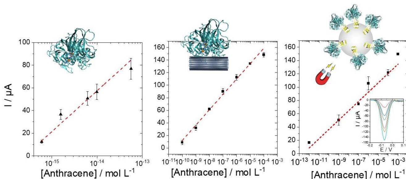
Figure 6. Linear part of the logarithmic plot of the SWV peak current towards anthracene concentration for the detection of anthracene at MWCNT electrode from (A) a solution of 1 \text{ U mL}^{-1} of laccase and 20 \text{ mM ABTS} left to react for 1 \text{ h} at 25^\circ\text{C} min, (B) from a POXA1b-modified MWCNT electrode in a solution of anthracene left to react for 2 \text{ h} at 40^\circ\text{C} and (C) a solution of 20 \text{ mU mL}^{-1} of biofunctionalized microbeads and 50 \text{ mM ABTS} left to react for 1 \text{ h} at 25^\circ\text{C} min (inset: corresponding SWV performed in a 0.1 \text{ M} phosphate/citrate buffer solution pH 5)
