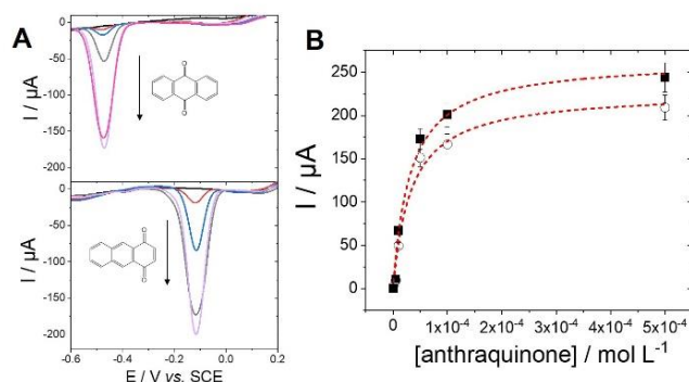
Figure 2. (A) SWV (0.1 M McIlvaine buffer pH 5, 25°C, pulse height = 25 mV, pulse width = 0.5 s, step height = -5 mV) performed after incubation (10 min, 25°C) of the MWCNT electrode in a MeCN solution of (a) 9,10-anthraquinone and (b) 1,4-anthraquinone at different concentrations
